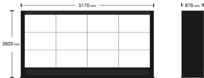
Full MultiTaction® iWall system (MTIW-3x4)
