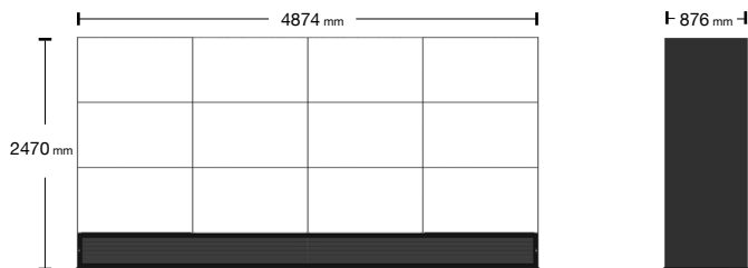
MultiTaction® iWall system in open frame configuration (MTIW-3x4OFO option used)
